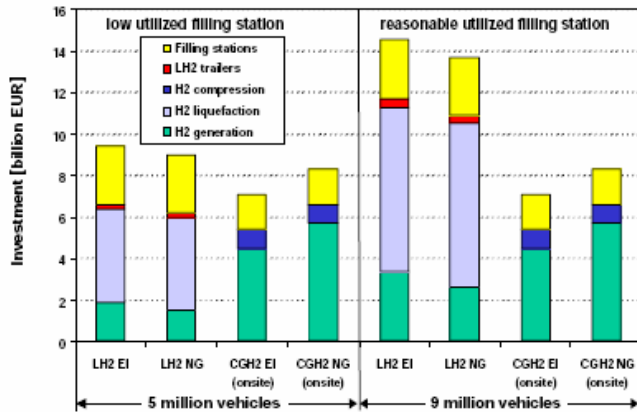
Figure 8 Investment for a transport hydrogen infrastructure from: Report of the Contact Group on Alternative Fuels, Annex 4 (compiled by HyNet)
